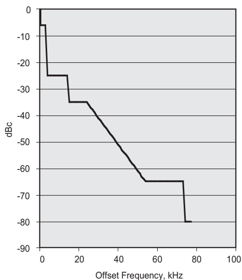
Figure 2. Spectrum Mask for AM stations running power levels >5000 watts.
