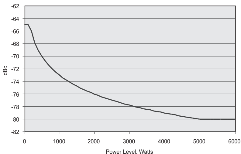
Figure 3. Allowed emission levels at offsets > 75 kHz.
