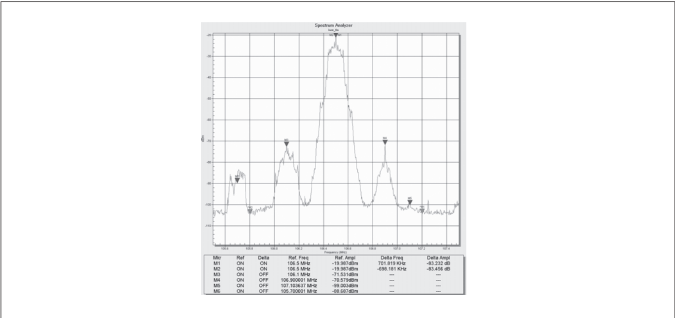
Figure 7. Measurement of Occupied Bandwidth on a broadcast FM signal.
