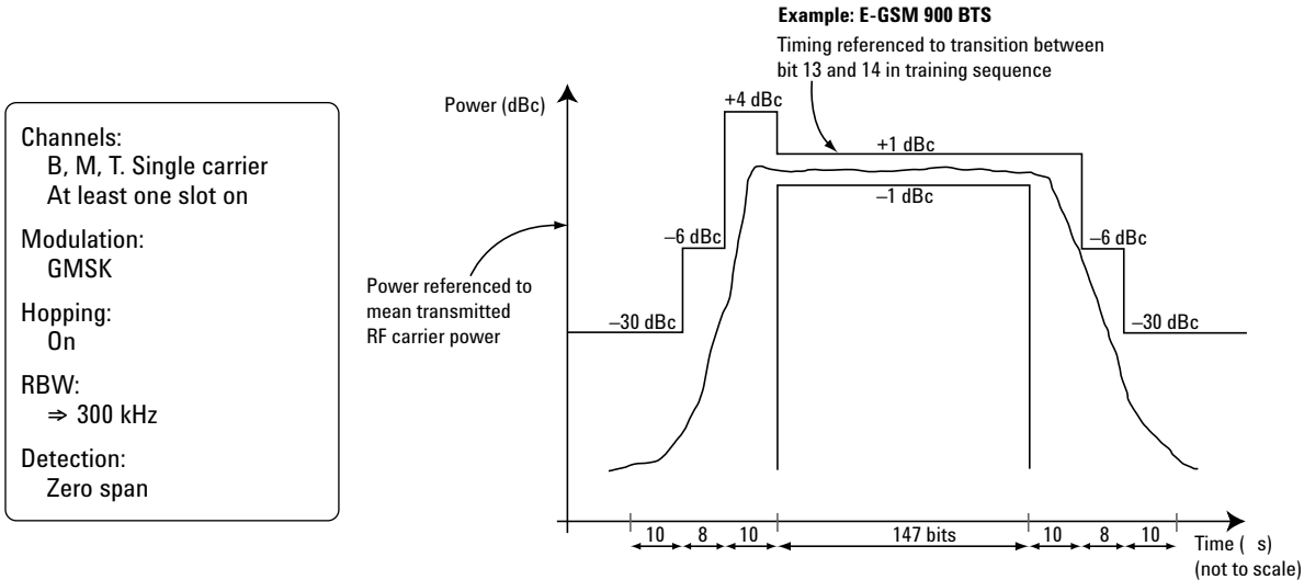
Figure 14. GMSK transmitted RF carrier power versus time, BTS, limits, GMSK
