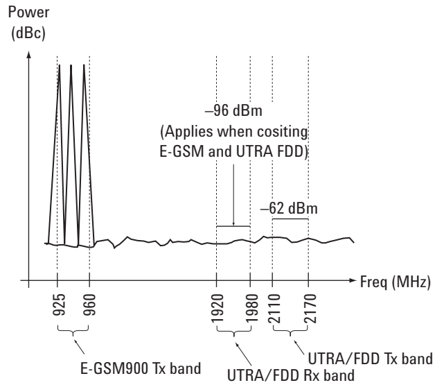
Figure 27. Cross band spurious. GSM900 into 3G bands, BTS, limits
