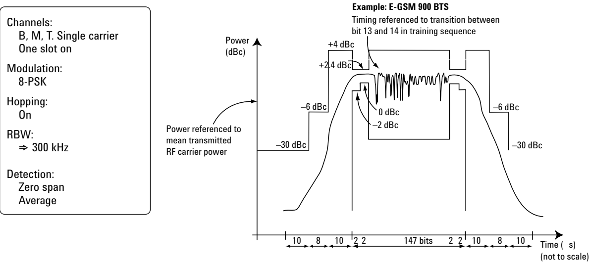
Figure 15. Transmitted RF carrier power versus time, BTS, limits: 8-PSK
