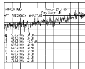
Figure 3. Correction factors.
