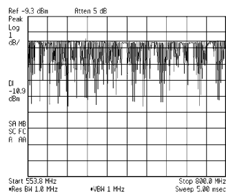
Figure 4. Corrected signal.
