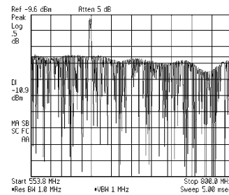
Figure 2. Original signal.
