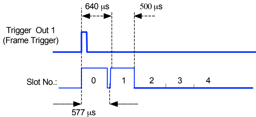
Figure 3: Setting for measuring the power of slot 1
