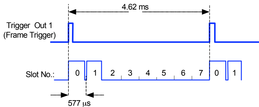
Figure 2: GSM/EDGE timing, slot 0 and slot 1 active
