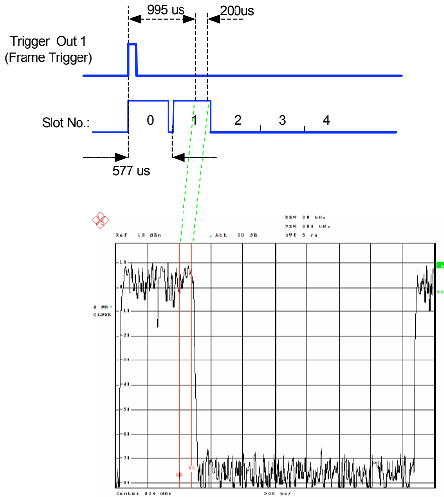
Figure 5: Setting of gate delay (0.995 ms) and gate length (0.2 ms) to measure the modulation spectrum of the 2nd timeslot (50 to 90% of the burst excluding the midamble)
