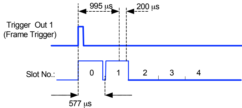
Figure 4: Setting for measuring the modulation spectrum of slot 1
