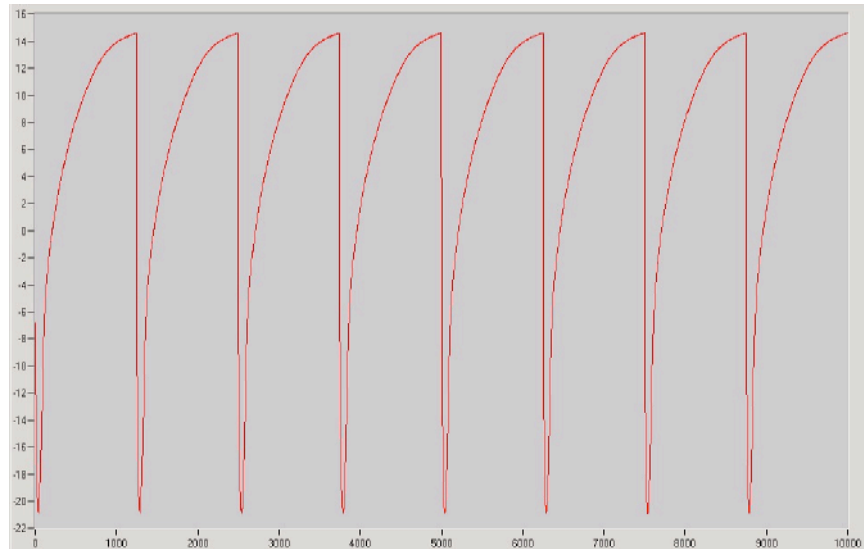
Figure 7: Graph of typical trace readout of gated measurements over 8 successive power rampings (power in dBm)
