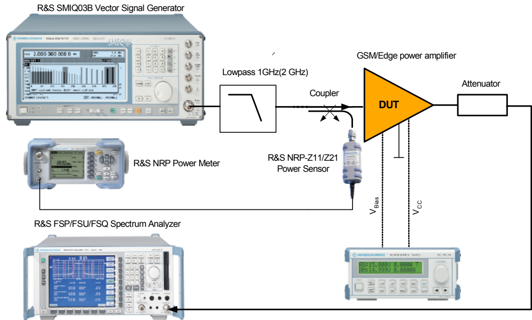
Figure 1: Typical test setup for testing GSM/EDGE mobile power amplifiers
